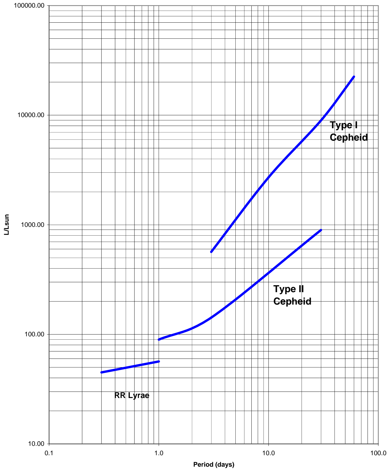
Luminosity vs Period
