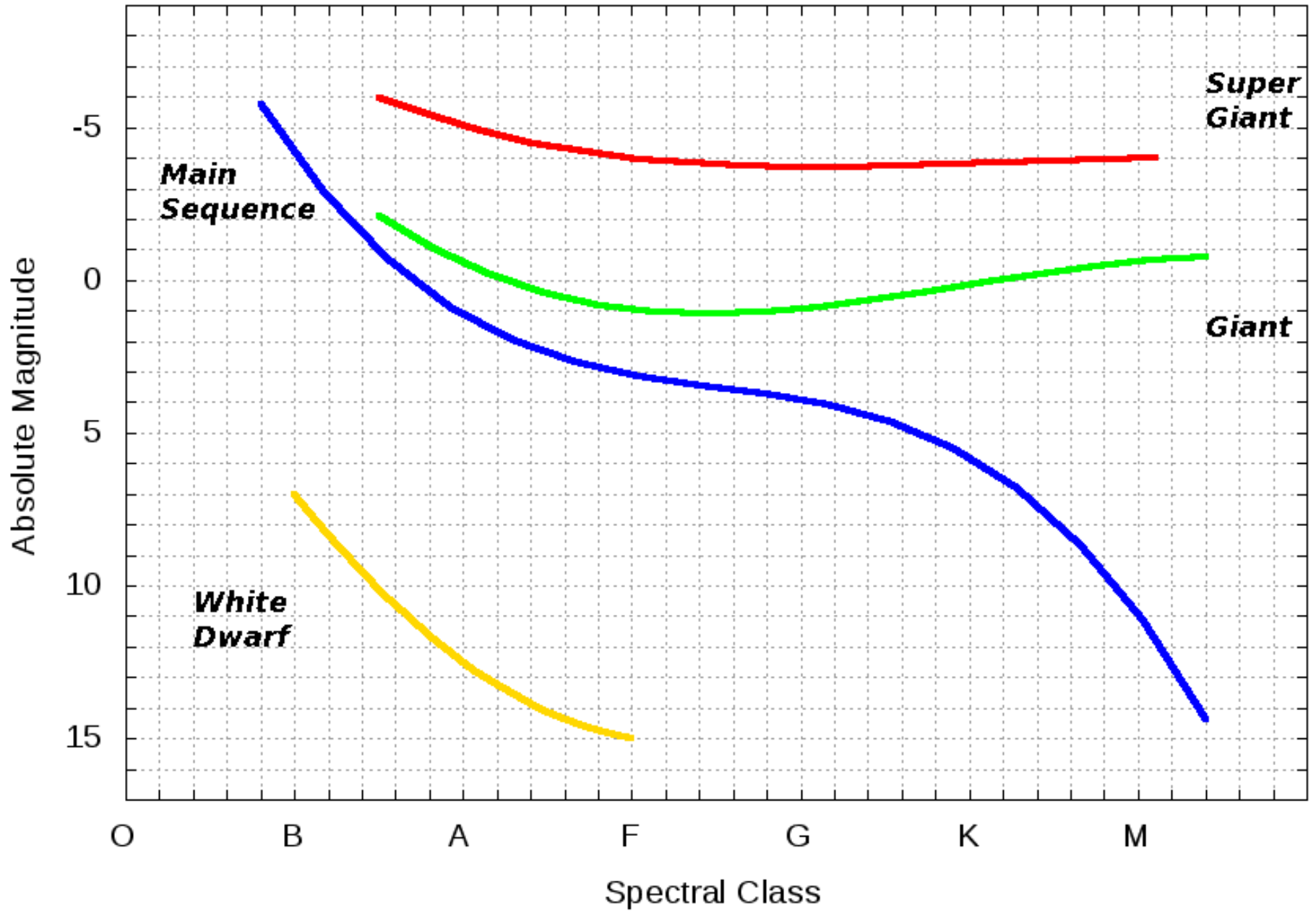
HR Diagram
